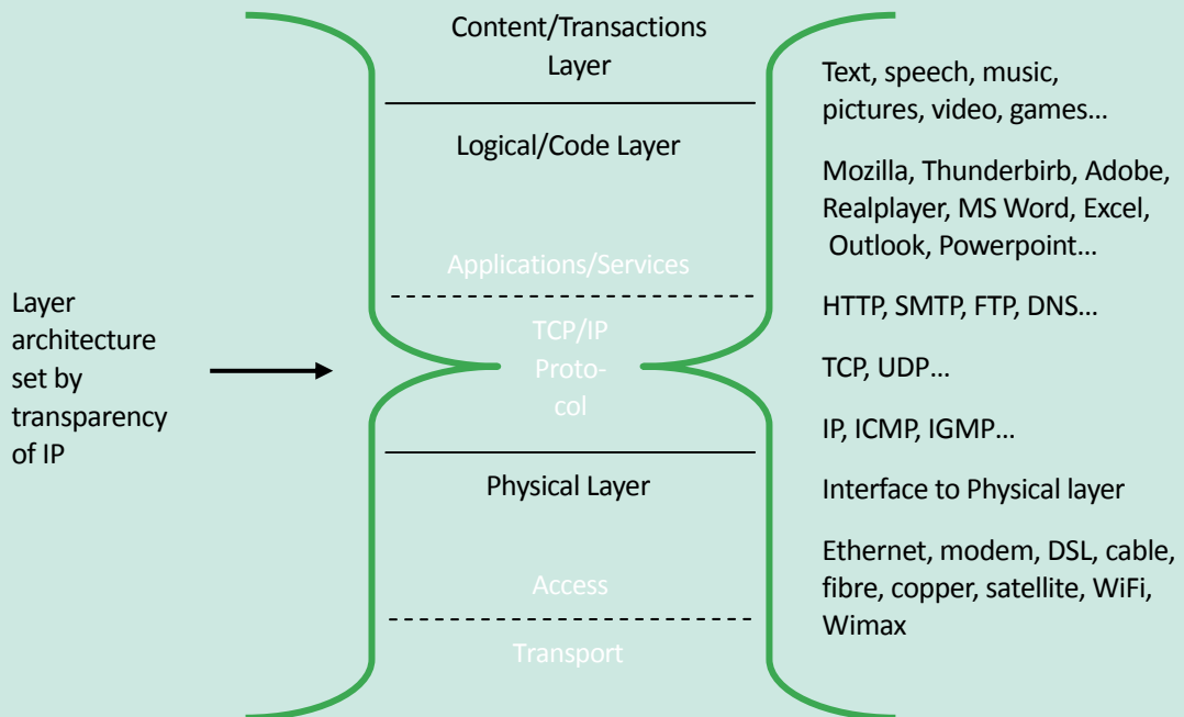
Figure 2.1: The Network Layer Model
